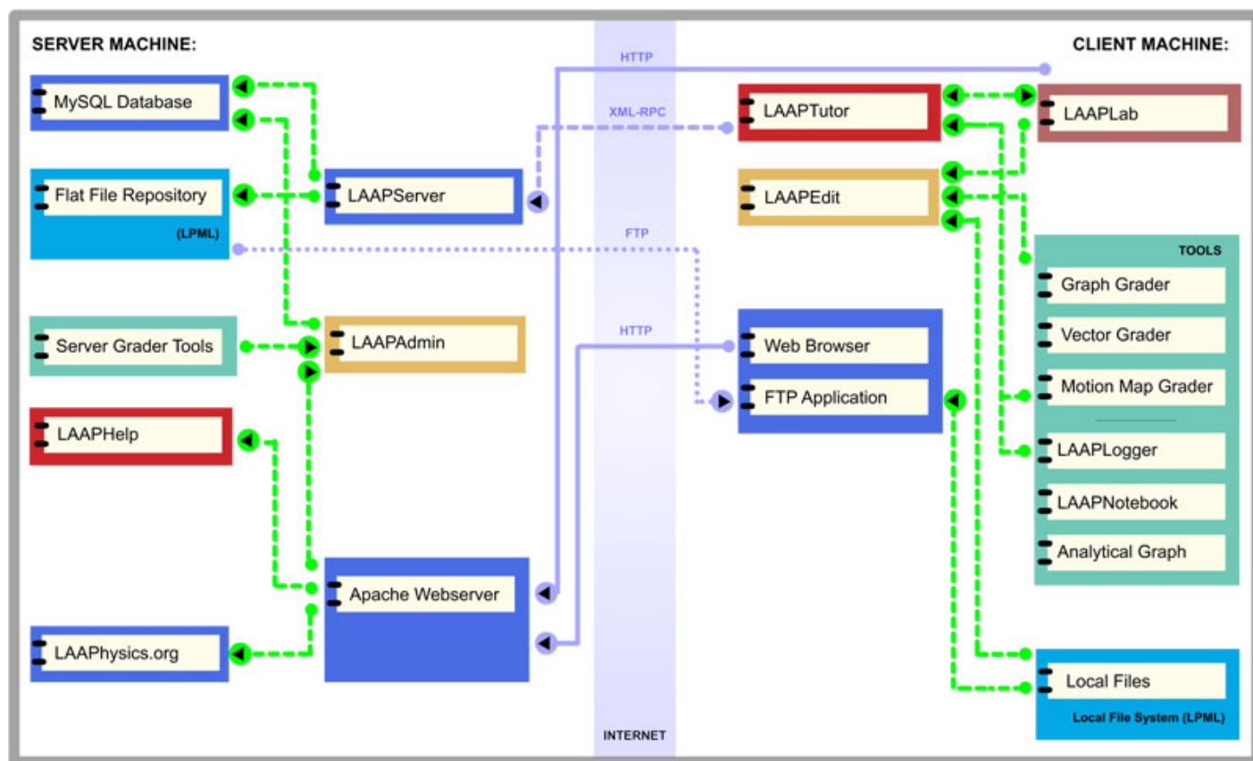
FIGURE 1. LabPhysics Architecture Schematic.
