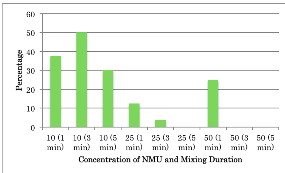
Figure 6: Comparison of percentage of pale green colored shoots appeared after 3 weeks of vortex mixing. Concentration is stated in \mu\text{M} .
