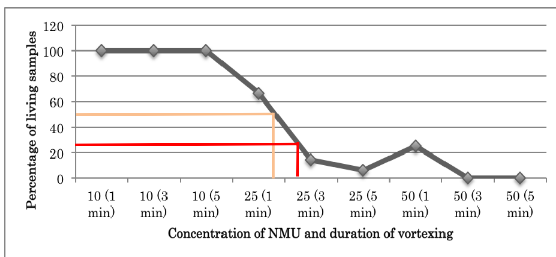
Figure 2: Result of vortex mixing (vortexing) mediated mutagenesis. Concentration of NMU is on \mu\text{M} . Lethal dosage of 75% ( \text{LD}_{75} ) is shown in red lines, while lethal dosage of 50% ( \text{LD}_{50} ) is shown in orange lines.
