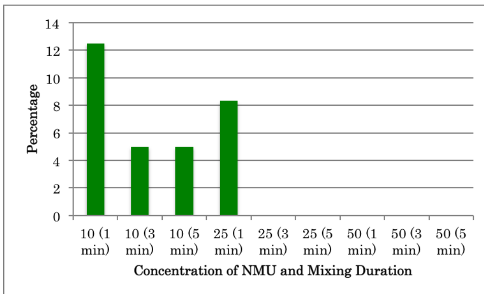
Figure 5: Comparison of percentage of green colored shoots appeared after 3 weeks of vortex mixing. Concentration is stated in \mu\text{M} .
